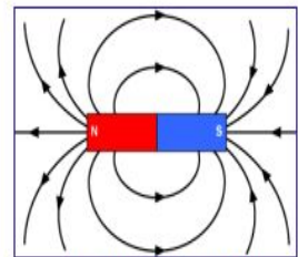
Magnetic Field
